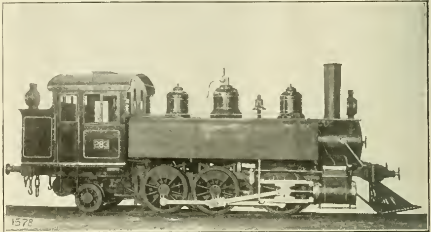
SIX COUPLED TANK LOCOMOTIVE FOR CHILI.
